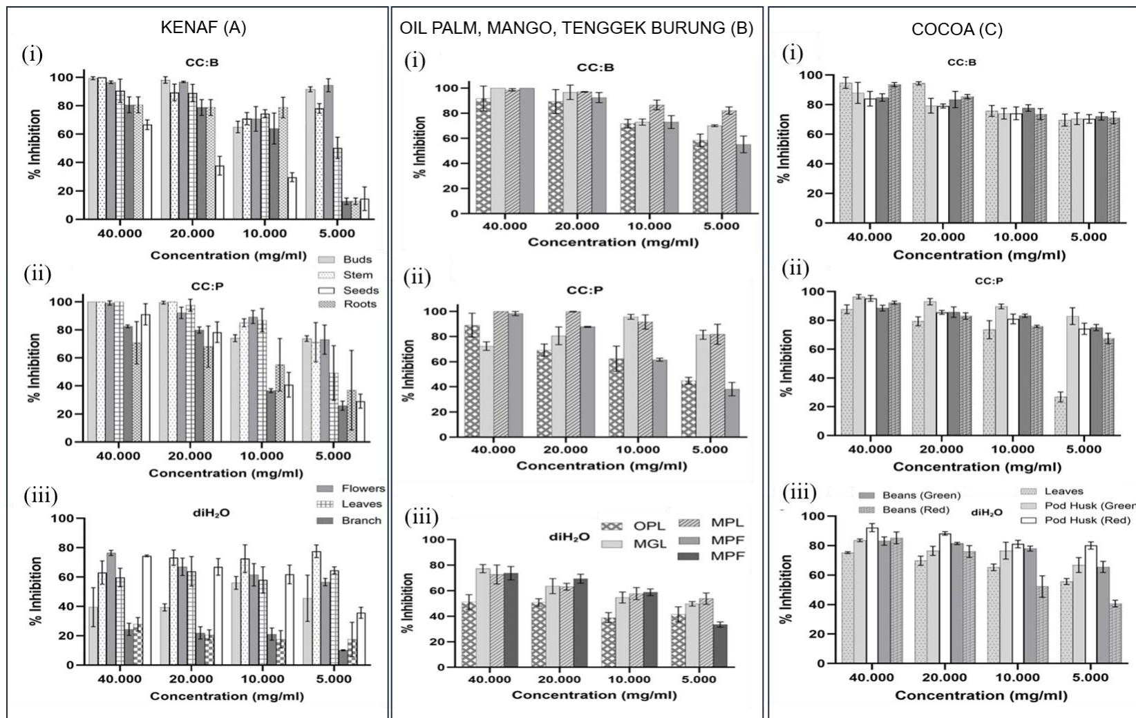
Figure 4. (A) Percentage inhibition of DPPH radical scavenging activity in various parts of kenaf; (B) Tenggek Burung, mango, and oil palm and (C) cocoa. Abbreviations: MPL: Melicope leaves, MPF: Melicope fruits, MGL: Mango leaves, OPL: Oil palm leaves.
